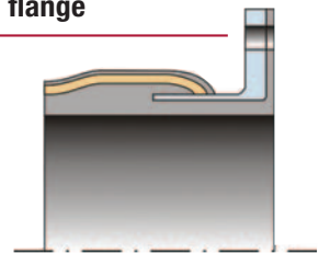
Part No.: xxxxx4 Vulcanized in steel nipple with rubber lining and fixed flange
