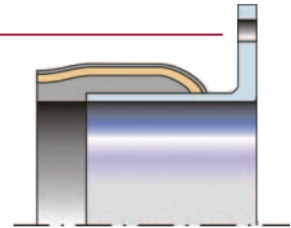
Part No.: xxxxx2 Vulcanized in steel nipple with fixed flange
